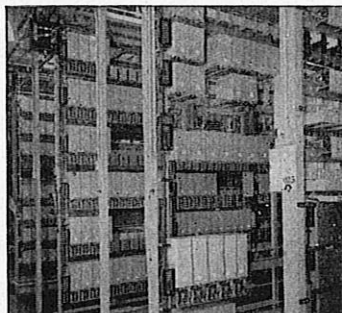
EXCHANGES (Telephone & Teleprinter)
